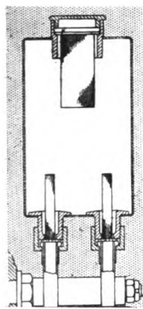
Pierce Oil Strainer.
